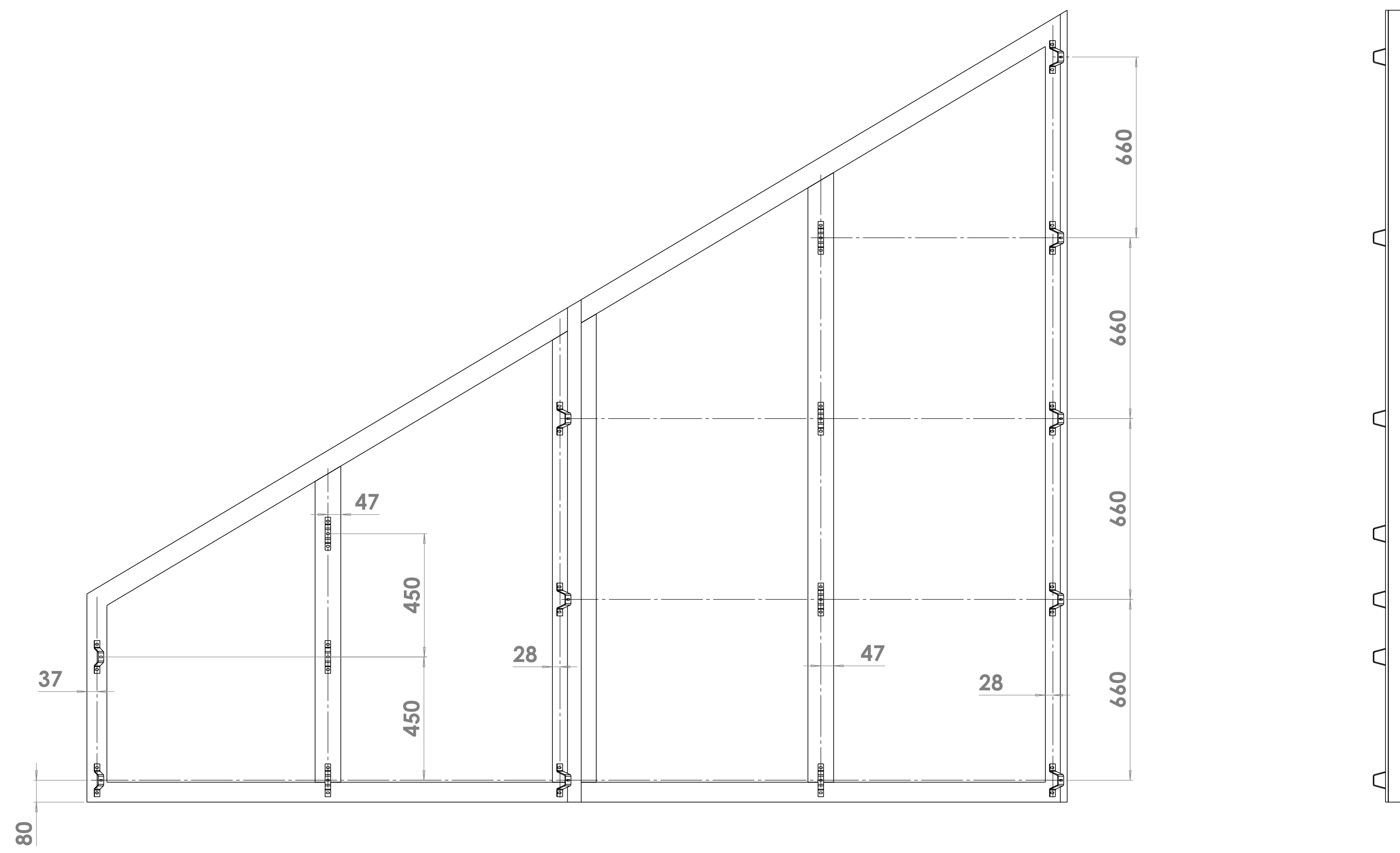
WINDOW FRAME (WITH BRACKETS)
